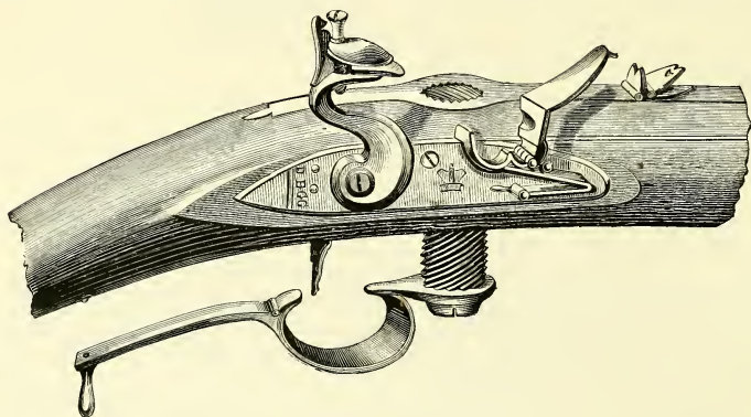
Fergusson Breech-loading Rifle.
